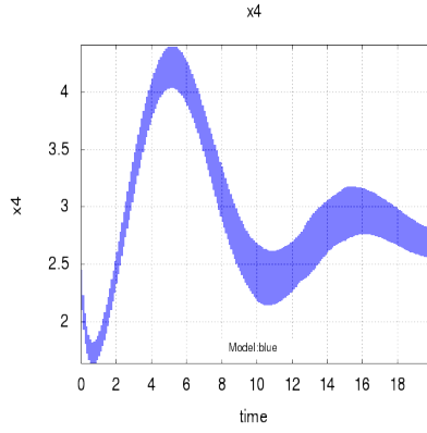
(c) C2E2
