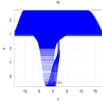
(c) C2E2.
