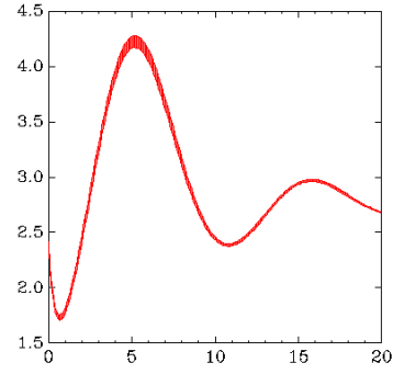
(b) CORA/SX
