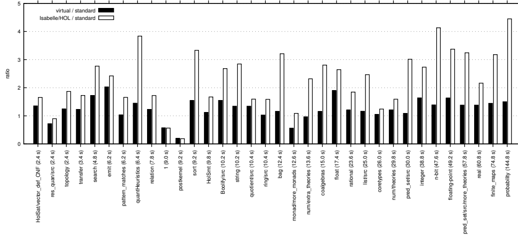
Figure 4 Performance measurements: HOL4 source directory on the x -axis, sorted by elapsed time (in parentheses) to build that directory with standard HOL4. Bars show the time (relative to standard HOL4) to build that directory with virtualized standard HOL4-Kernel (black) and the Isabelle HOL4-Kernel (white).
